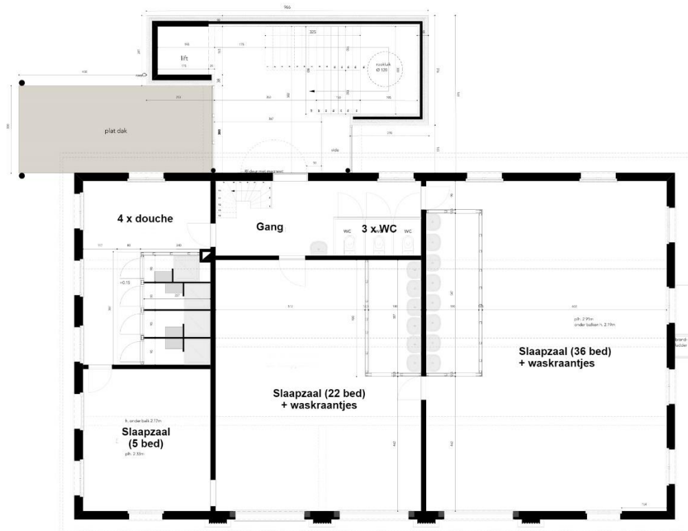
plan verdieping
